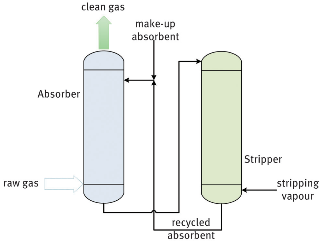
Figure 9: Absorption-stripping system.
